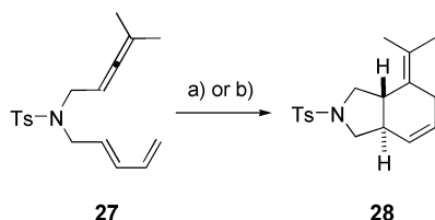
Scheme 3. Comparison of two gold phosphoramidite complexes in the asymmetric [4+2] cycloaddition of allene–diene 27 : a) [7·AuCl] (2 mol %), AgSbF 6 (2 mol %), CH 2 Cl 2 , –15 °C, 92 % yield, 92 % ee (Ref. [12a]), or b) 20b (5.5 mol %), AgBF 4 (5 mol %), CH 2 Cl 2 , 0 °C, 90 % yield, 91 % ee .
